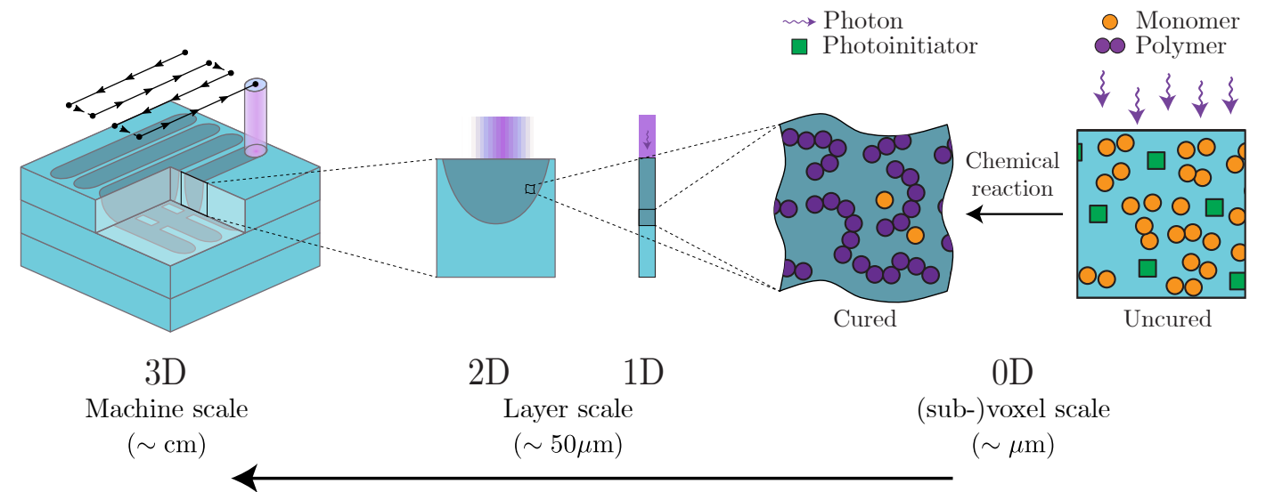
Figure 1: Bottom-up roadmap, ranging from a 0D (sub-)voxel to a full 3D product, illustrating the different scales to control the photopolymerization process.
